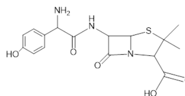
Figure 1. Chemical structure of amoxicillin (AMX).
